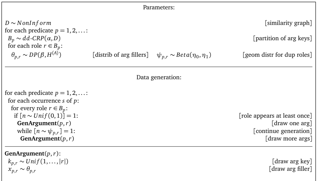
Figure 1: The BayesSRL model.
